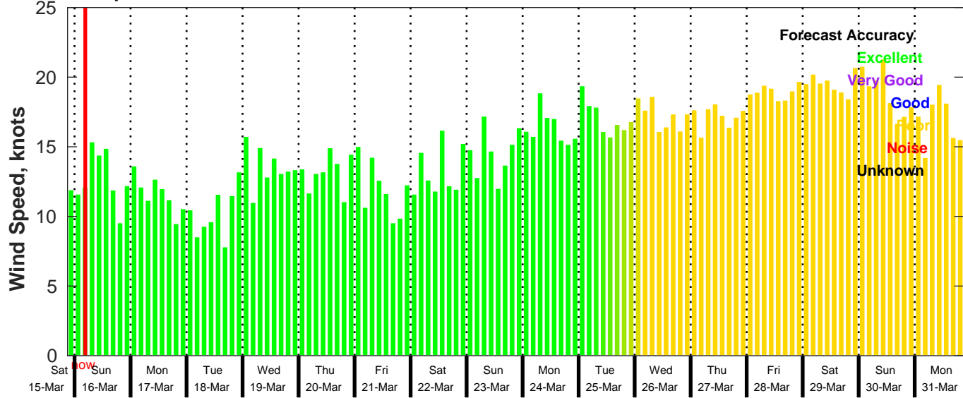
GFS Wind Speed Forecast for NDBC 41040 from 15-Mar-2025 21:00:00 to 31-Mar-2025 21:00:00
