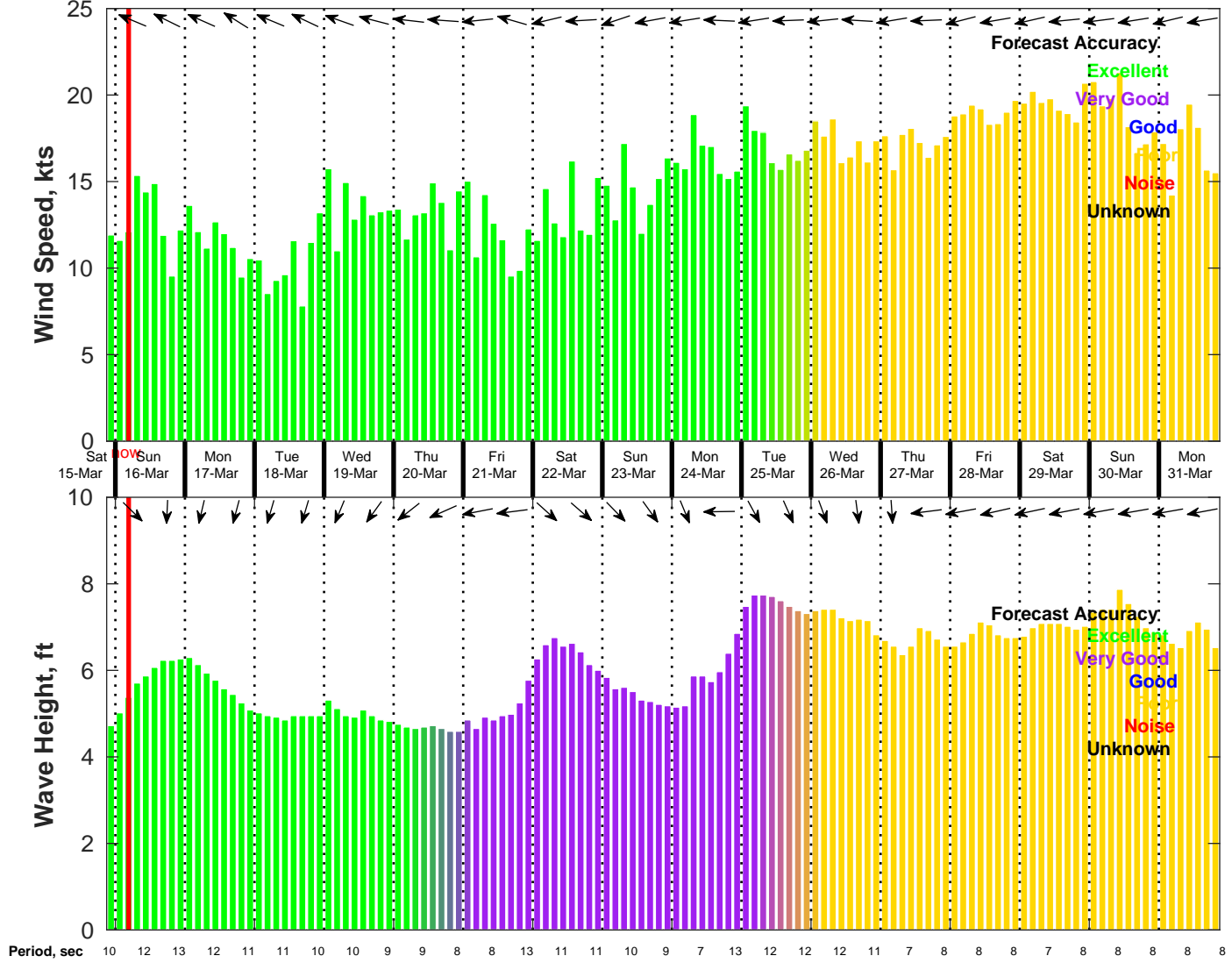
Wind & Wave Forecast for NDBC 41040 from 15-Mar-2025 21:00:00 to 31-Mar-2025 21:00:00
