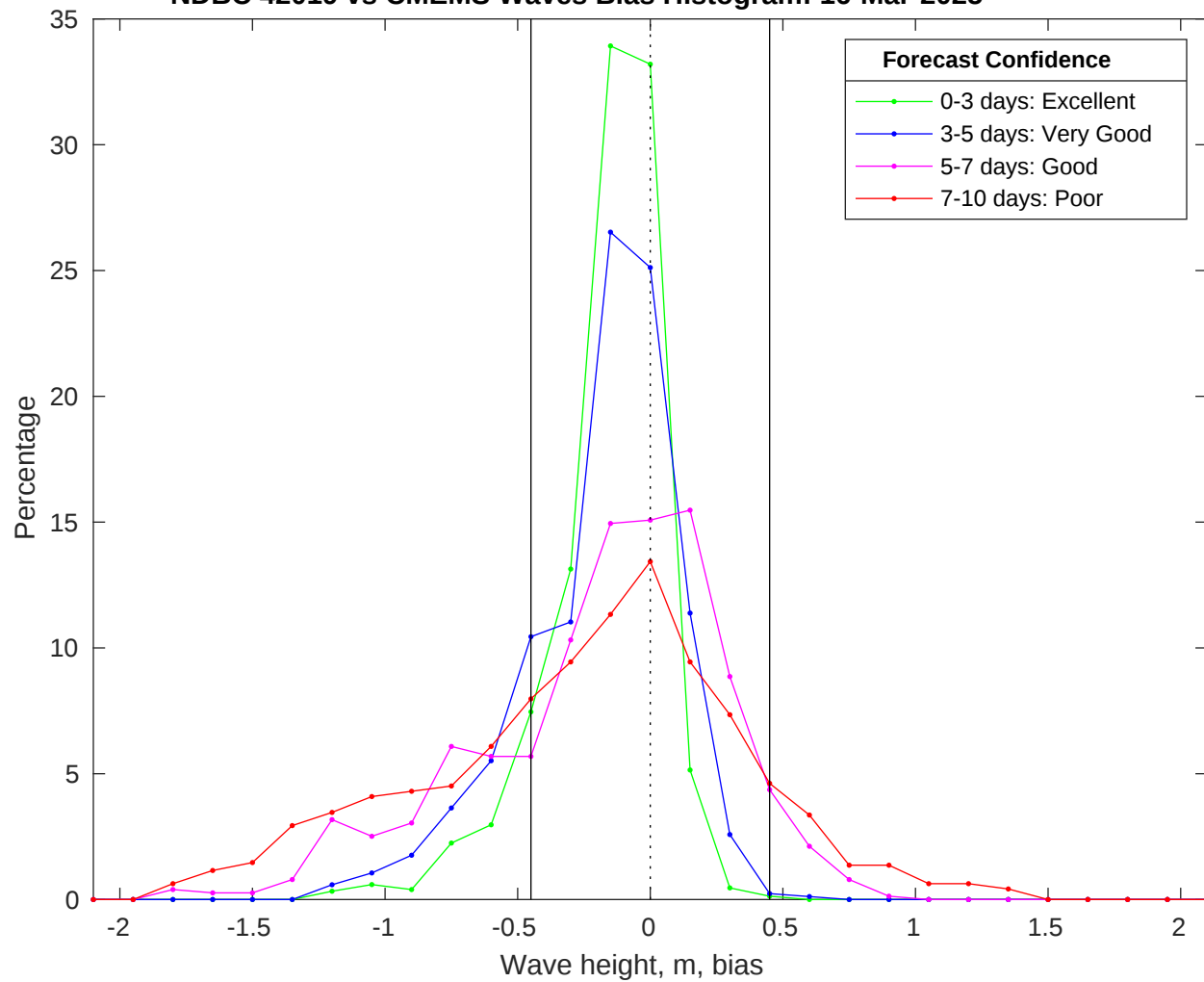
NDBC 42019 vs CMEMS Waves Bias Histogram: 16-Mar-2025
