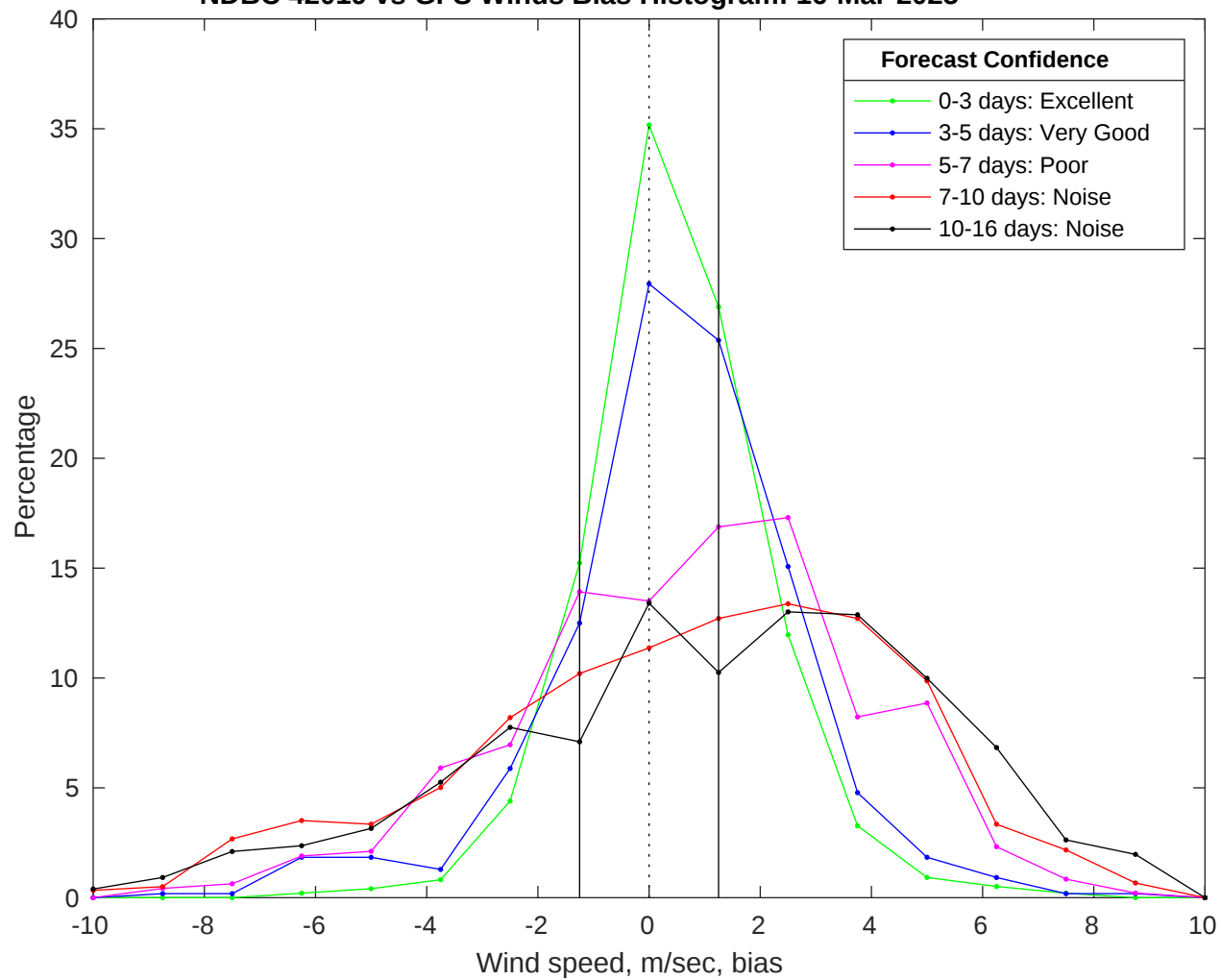
NDBC 42019 vs GFS Winds Bias Histogram: 16-Mar-2025
