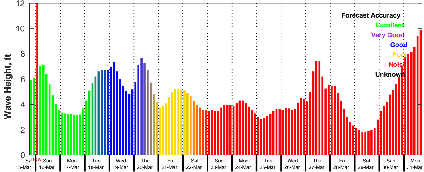
GFS Wave Forecast for NDBC 42019 from 15-Mar-2025 18:00:00 to 31-Mar-2025 18:00:00
