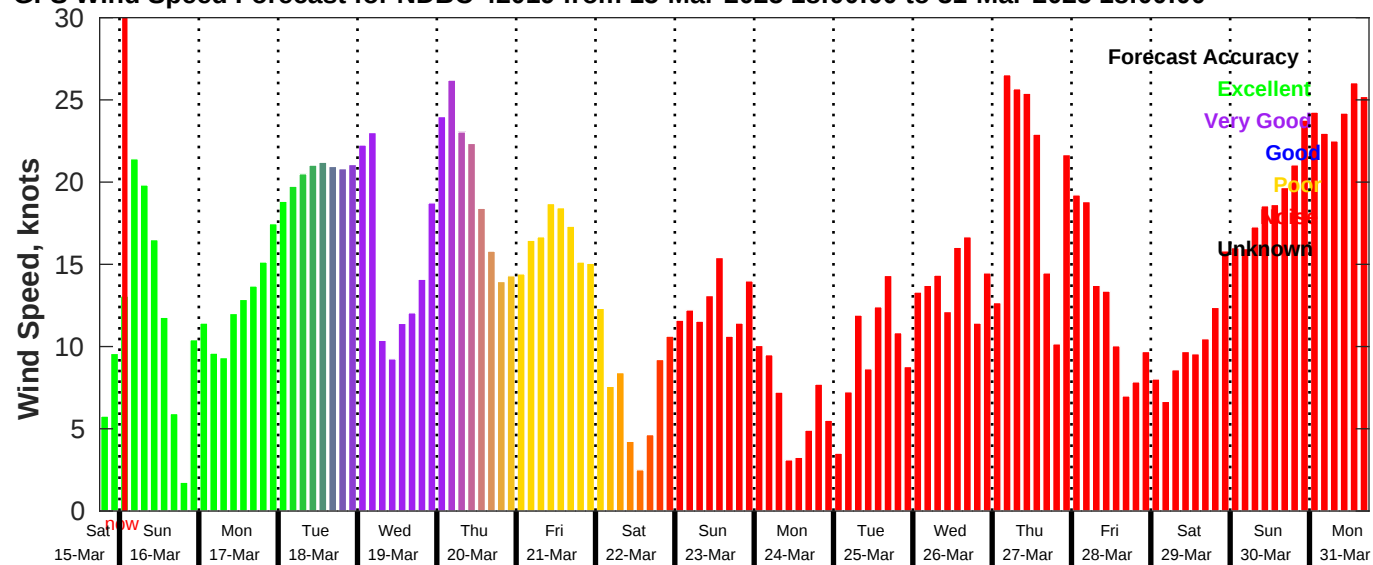
GFS Wind Speed Forecast for NDBC 42019 from 15-Mar-2025 18:00:00 to 31-Mar-2025 18:00:00
