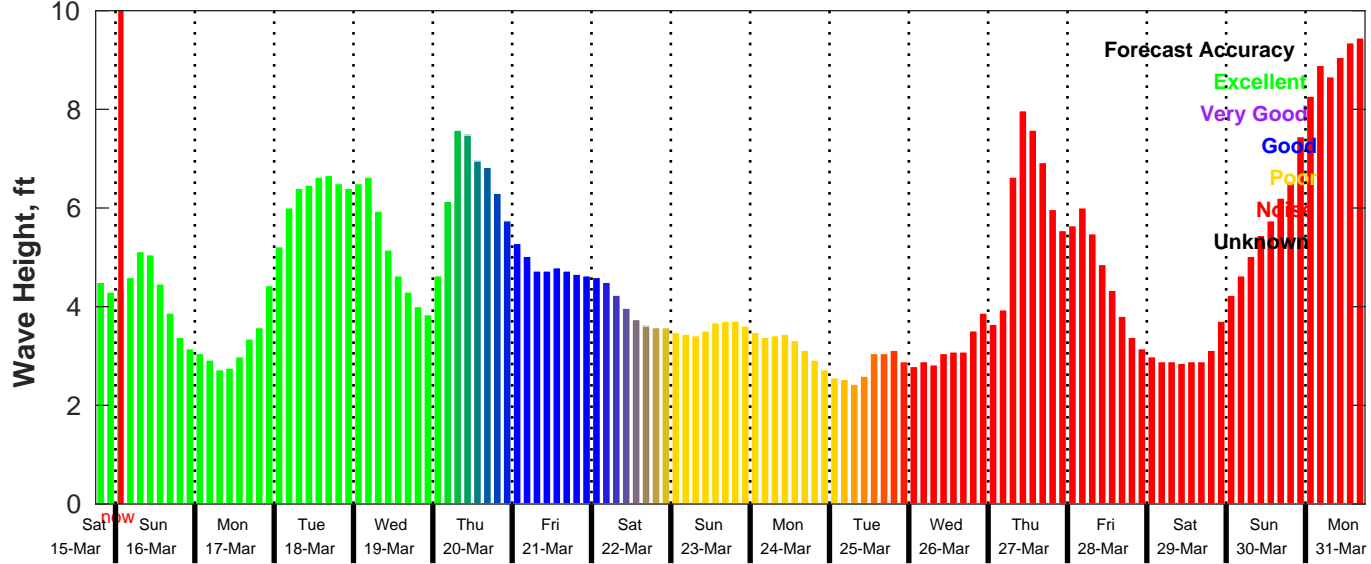
GFS Wave Forecast for NDBC 42020 from 15-Mar-2025 18:00:00 to 31-Mar-2025 18:00:00
