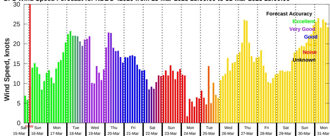
GFS Wind Speed Forecast for NDBC 42020 from 15-Mar-2025 18:00:00 to 31-Mar-2025 18:00:00
