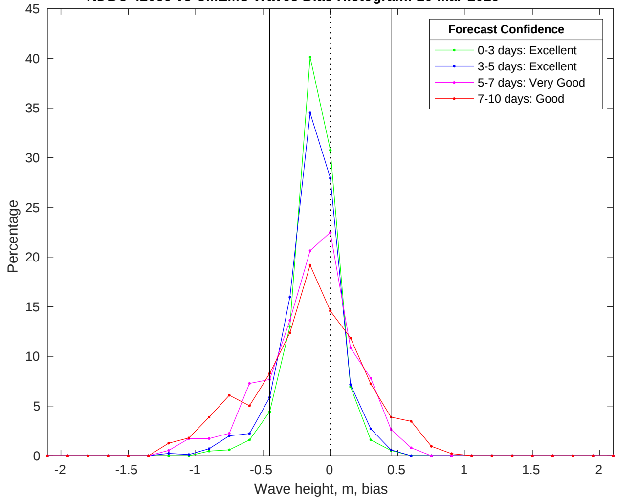
NDBC 42035 vs CMEMS Waves Bias Histogram: 16-Mar-2025
