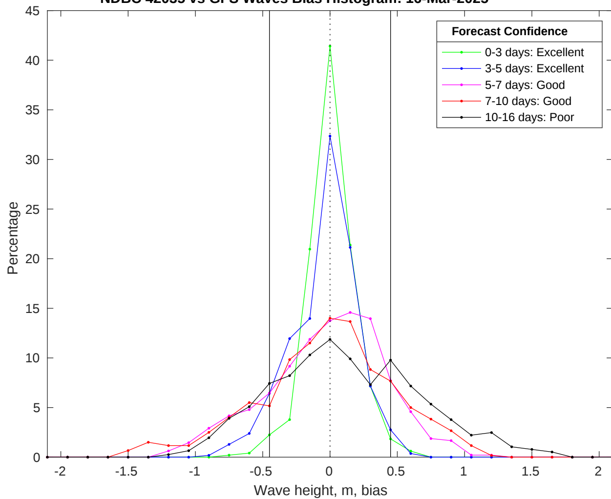
NDBC 42035 vs GFS Waves Bias Histogram: 16-Mar-2025
