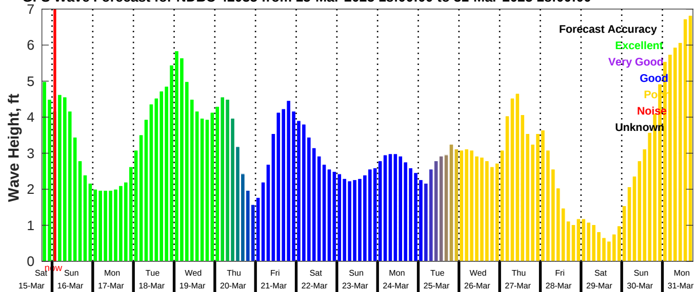
GFS Wave Forecast for NDBC 42035 from 15-Mar-2025 18:00:00 to 31-Mar-2025 18:00:00
