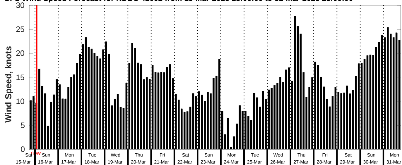
GFS Wind Speed Forecast for NDBC 42092 from 15-Mar-2025 18:00:00 to 31-Mar-2025 18:00:00
