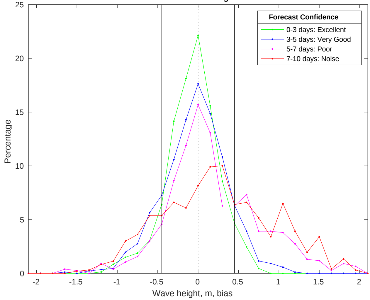
NDBC 46011 vs CMEMS Waves Bias Histogram: 16-Mar-2025
