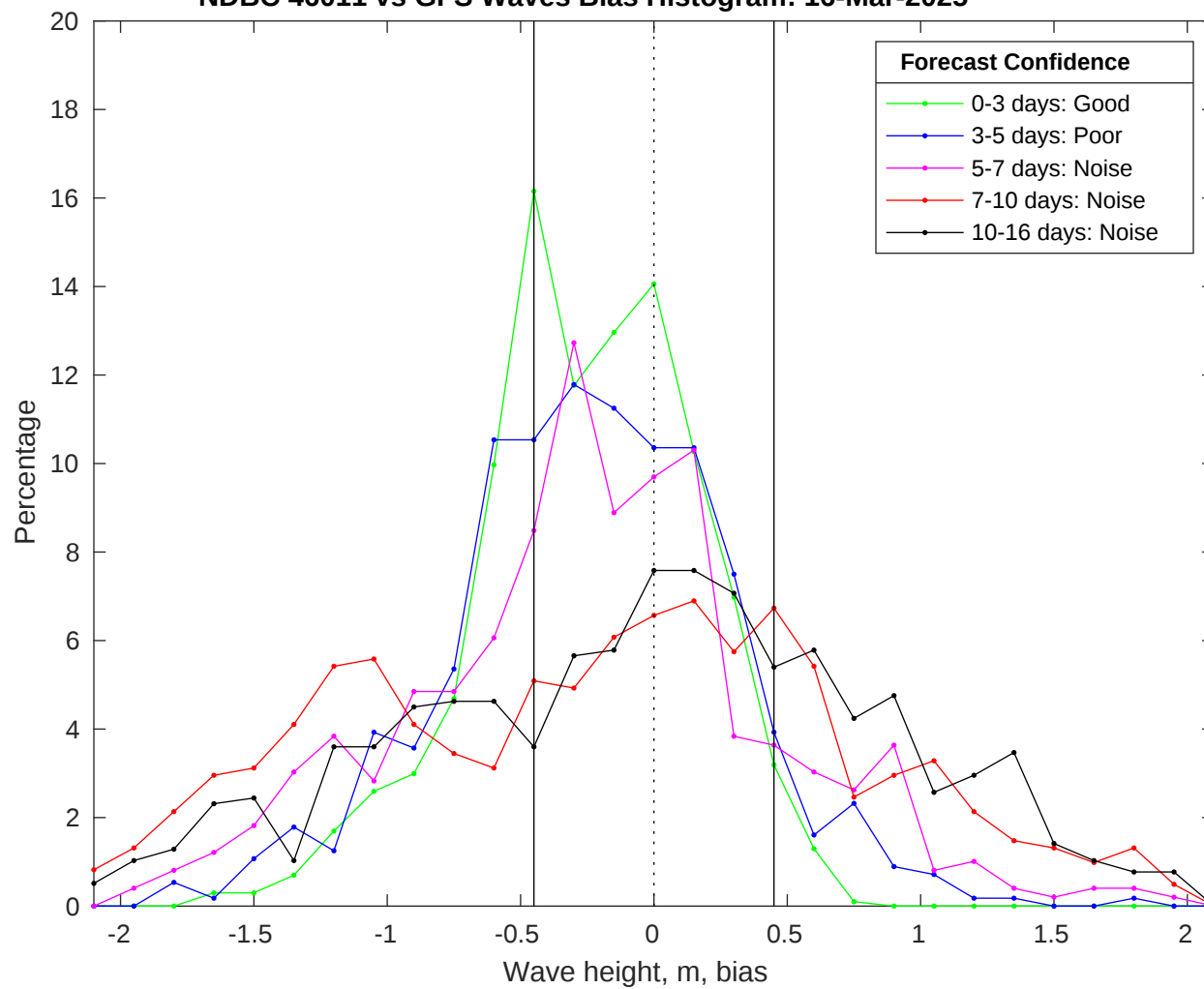
NDBC 46011 vs GFS Waves Bias Histogram: 16-Mar-2025
