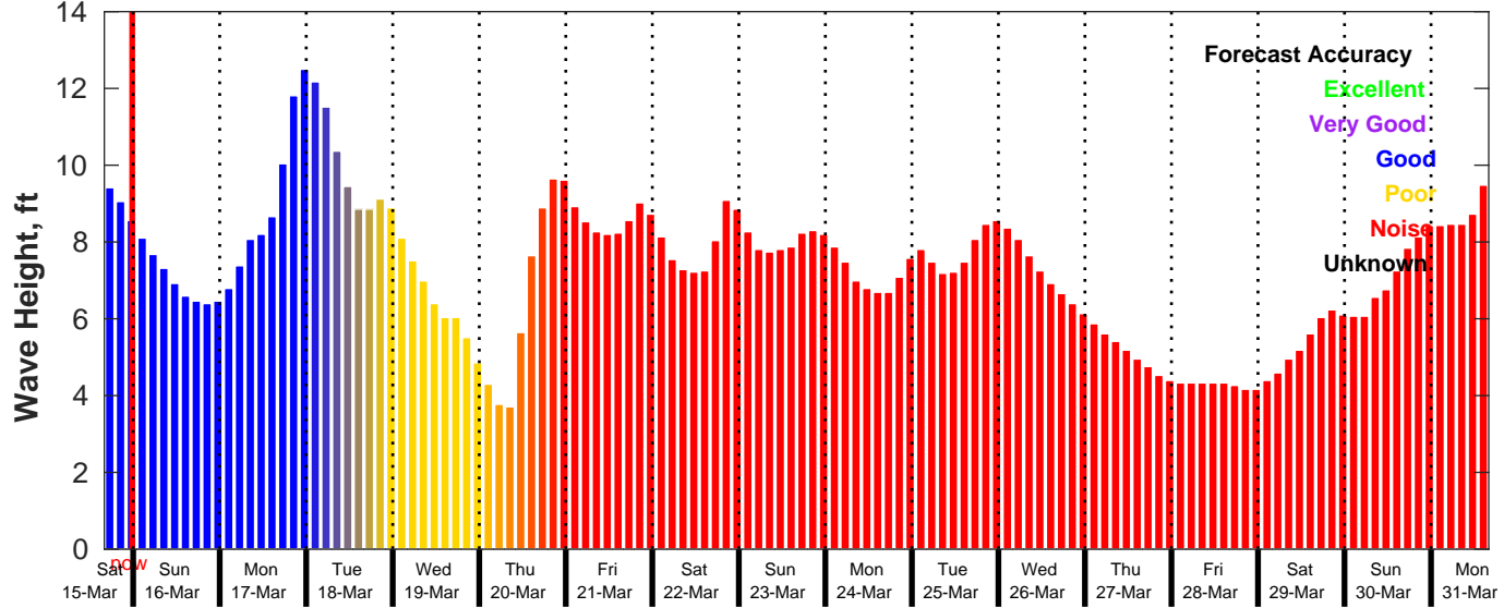
GFS Wave Forecast for NDBC 46011 from 15-Mar-2025 16:00:00 to 31-Mar-2025 16:00:00
