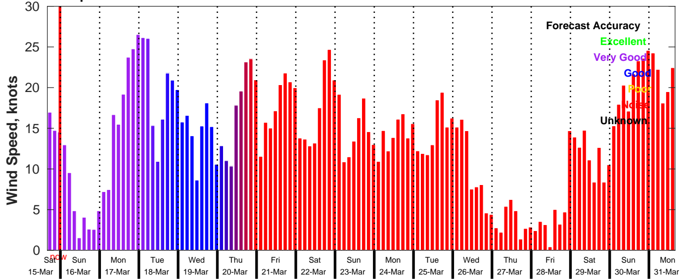
GFS Wind Speed Forecast for NDBC 46011 from 15-Mar-2025 16:00:00 to 31-Mar-2025 16:00:00
