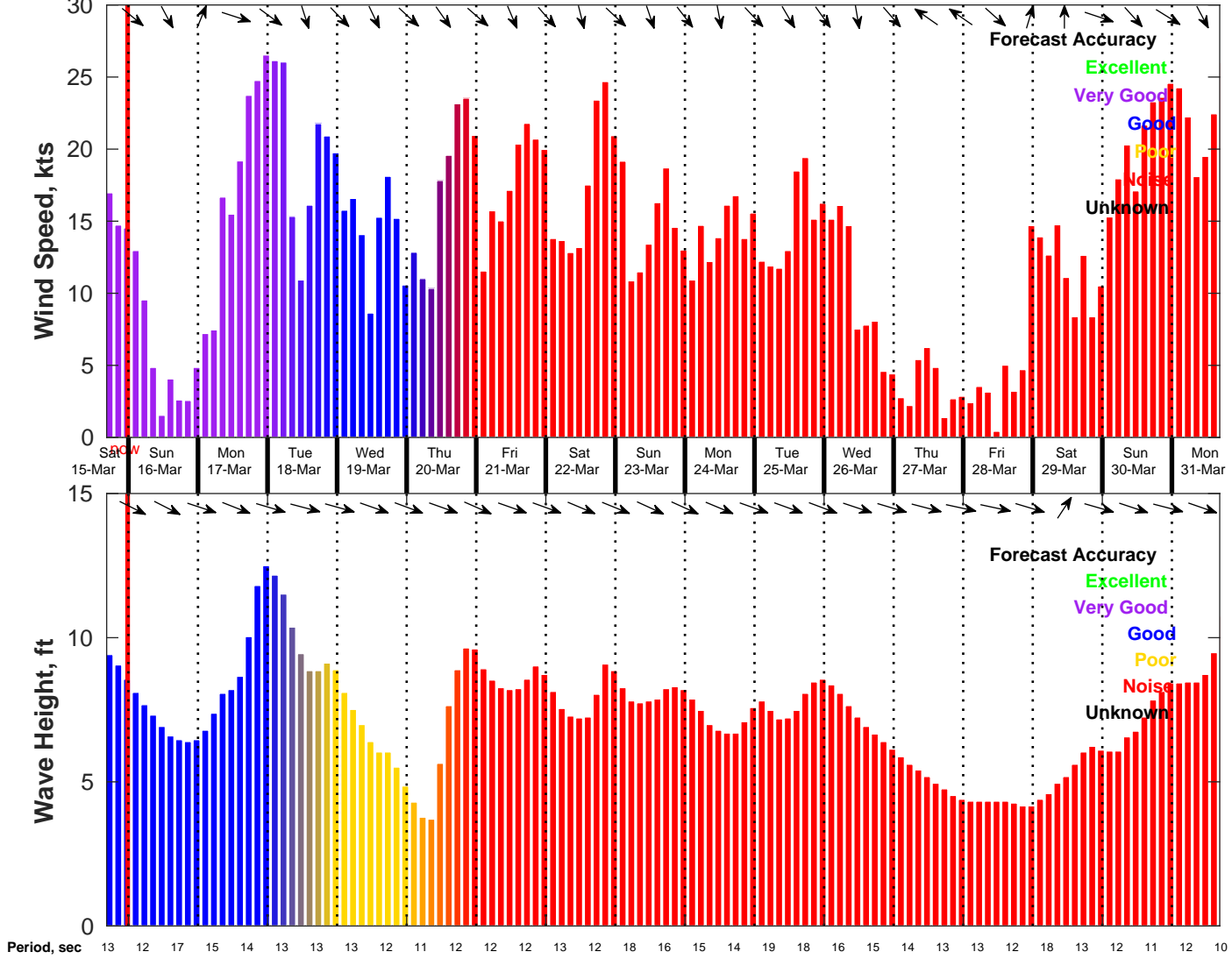
Wind & Wave Forecast for NDBC 46011 from 15-Mar-2025 16:00:00 to 31-Mar-2025 16:00:00
