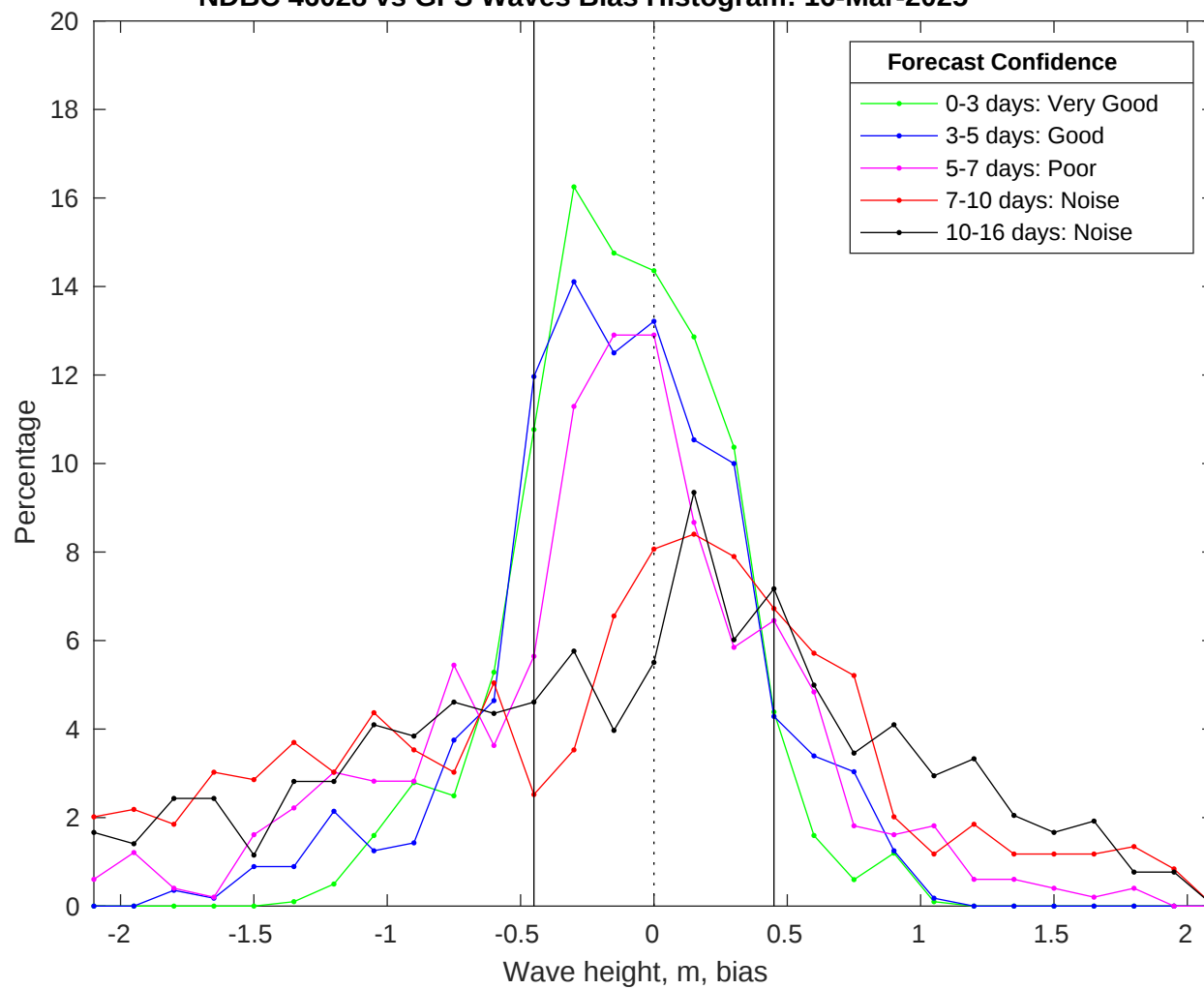
NDBC 46028 vs GFS Waves Bias Histogram: 16-Mar-2025
