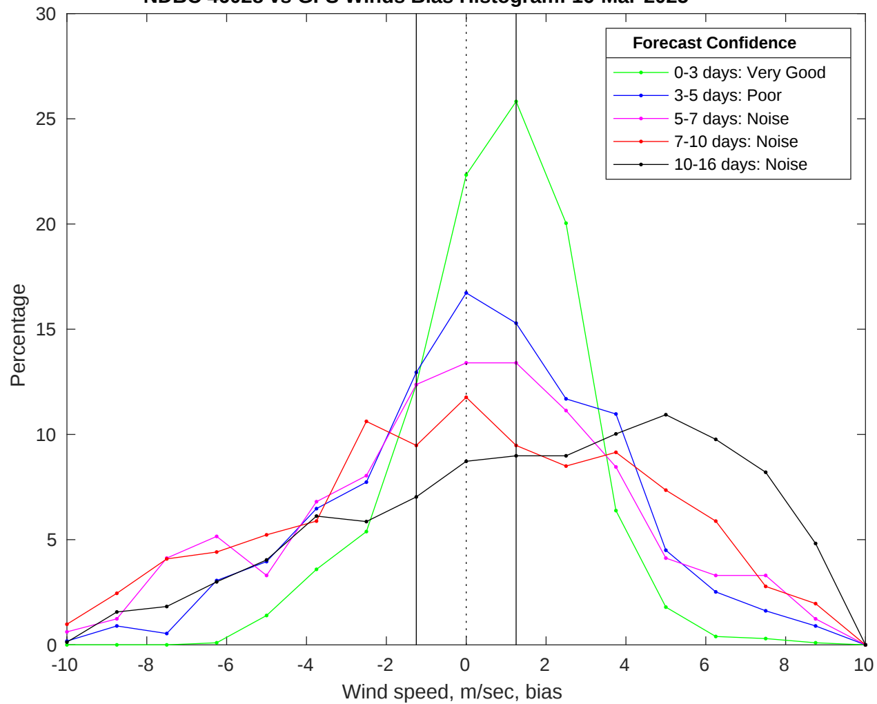
NDBC 46028 vs GFS Winds Bias Histogram: 16-Mar-2025
