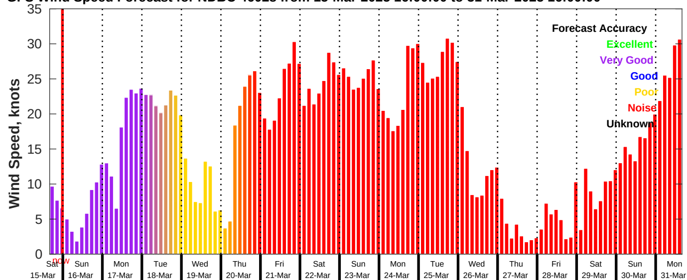
GFS Wind Speed Forecast for NDBC 46028 from 15-Mar-2025 16:00:00 to 31-Mar-2025 16:00:00
