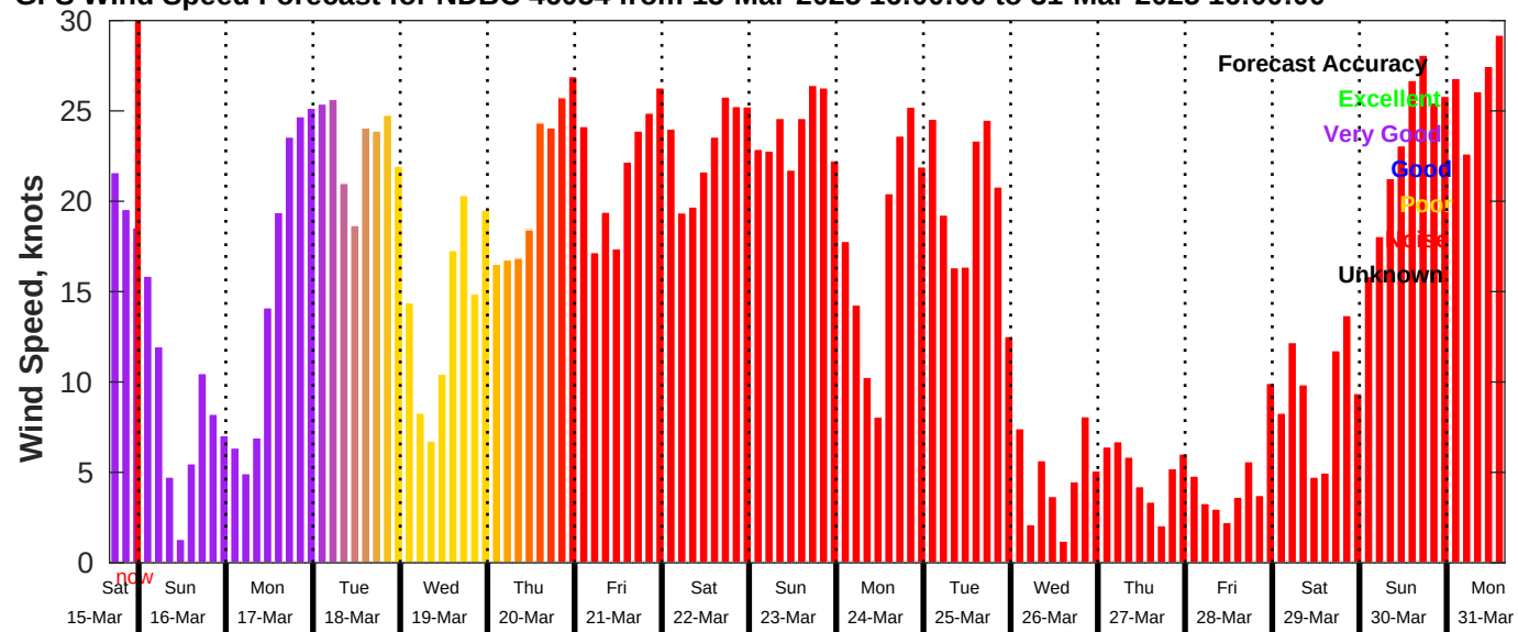
GFS Wind Speed Forecast for NDBC 46054 from 15-Mar-2025 16:00:00 to 31-Mar-2025 16:00:00
