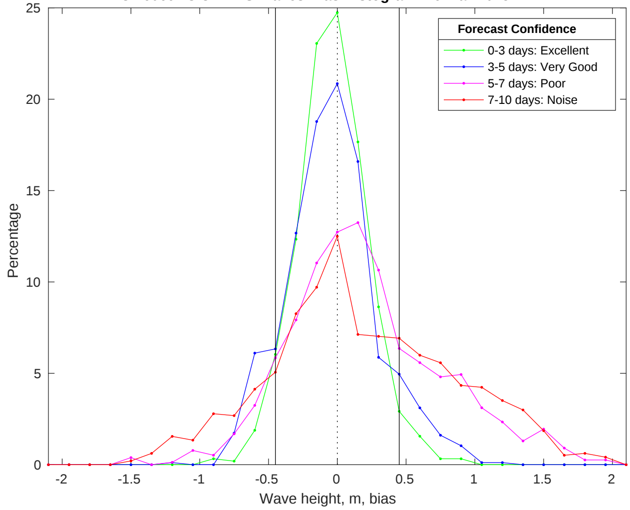
NDBC 46069 vs CMEMS Waves Bias Histogram: 16-Mar-2025
