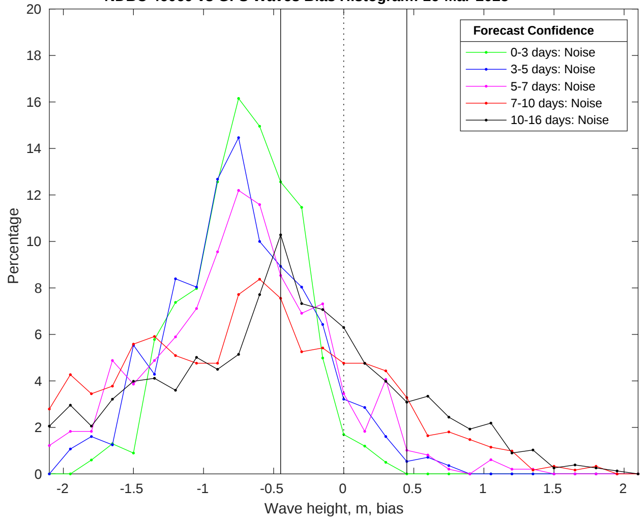
NDBC 46069 vs GFS Waves Bias Histogram: 16-Mar-2025
