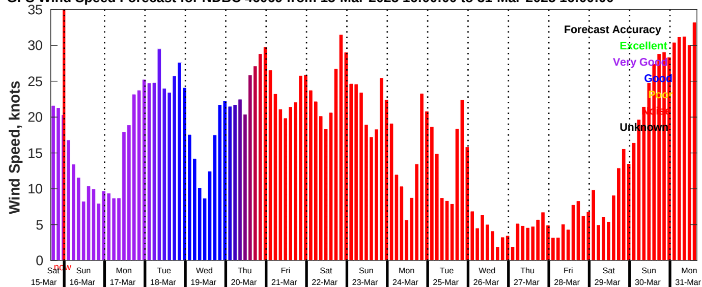
GFS Wind Speed Forecast for NDBC 46069 from 15-Mar-2025 16:00:00 to 31-Mar-2025 16:00:00
