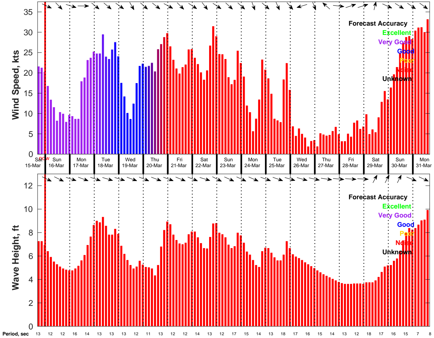
Wind & Wave Forecast for NDBC 46069 from 15-Mar-2025 16:00:00 to 31-Mar-2025 16:00:00
