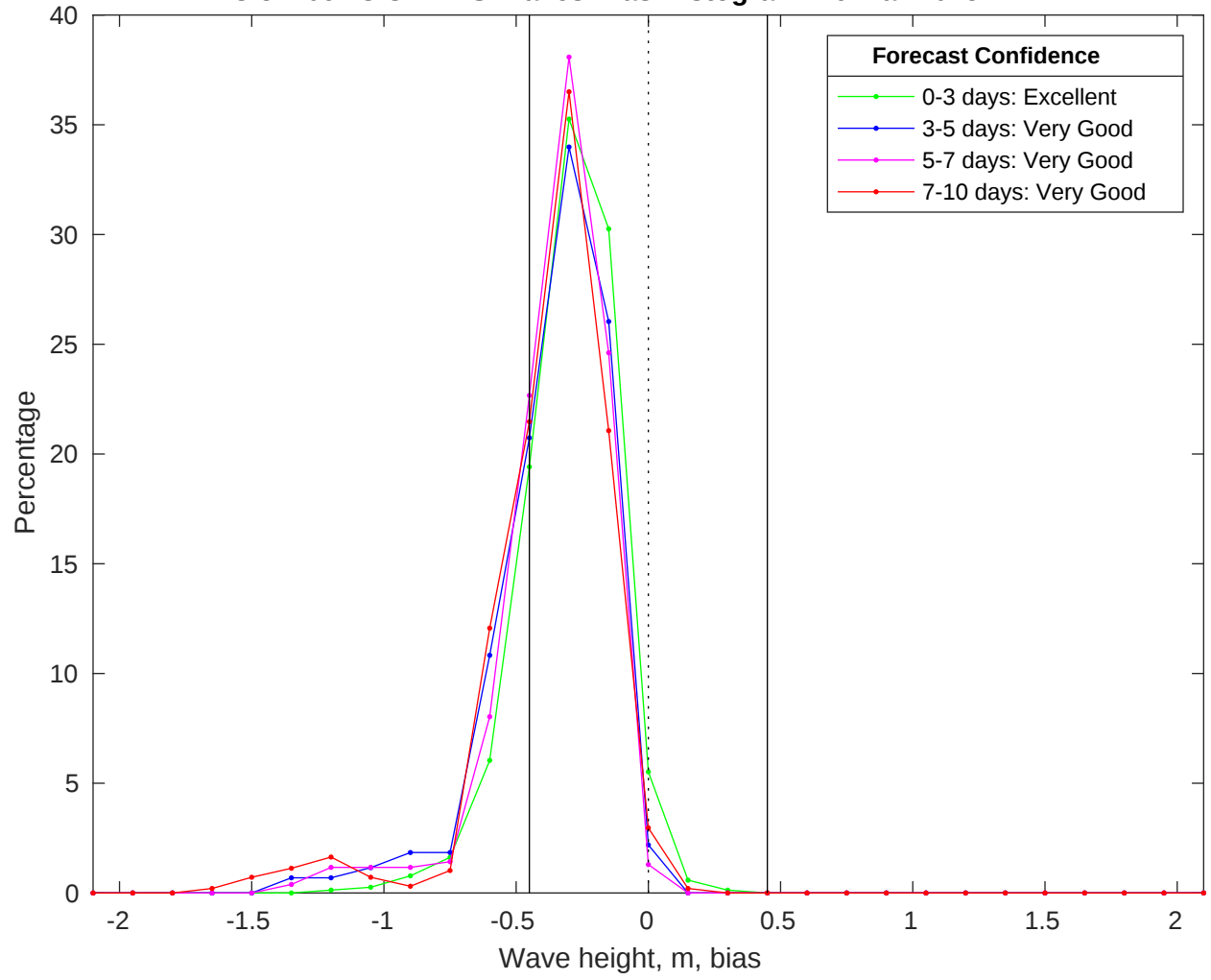
NDBC 51209 vs CMEMS Waves Bias Histogram: 16-Mar-2025
