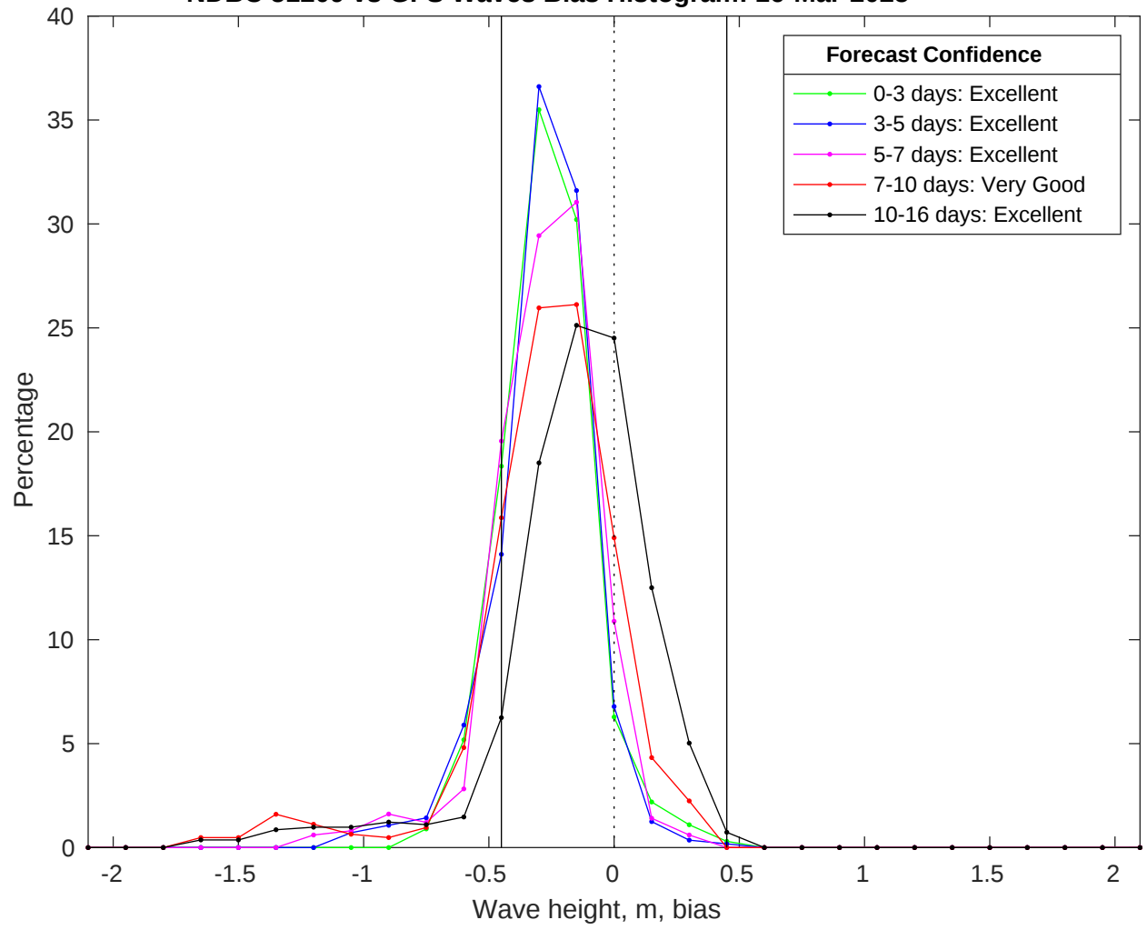
NDBC 51209 vs GFS Waves Bias Histogram: 16-Mar-2025
