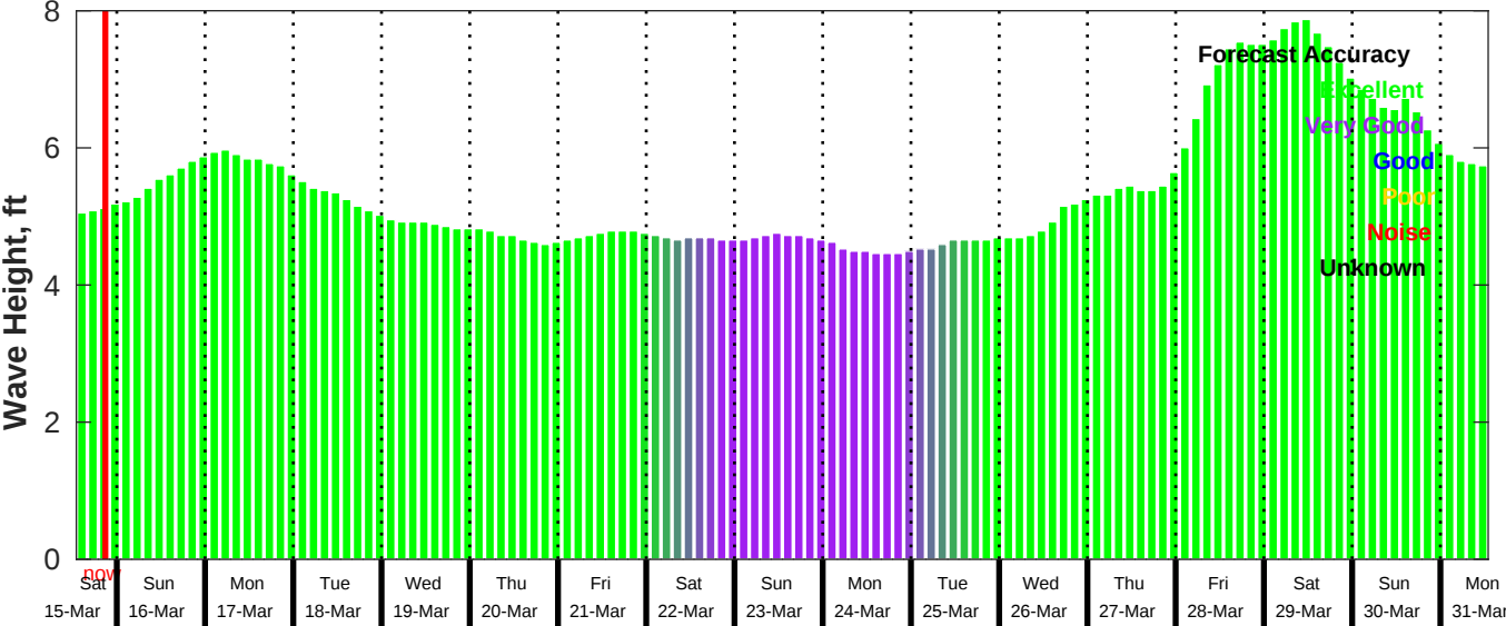
GFS Wave Forecast for NDBC 51209 from 15-Mar-2025 13:00:00 to 31-Mar-2025 13:00:00
