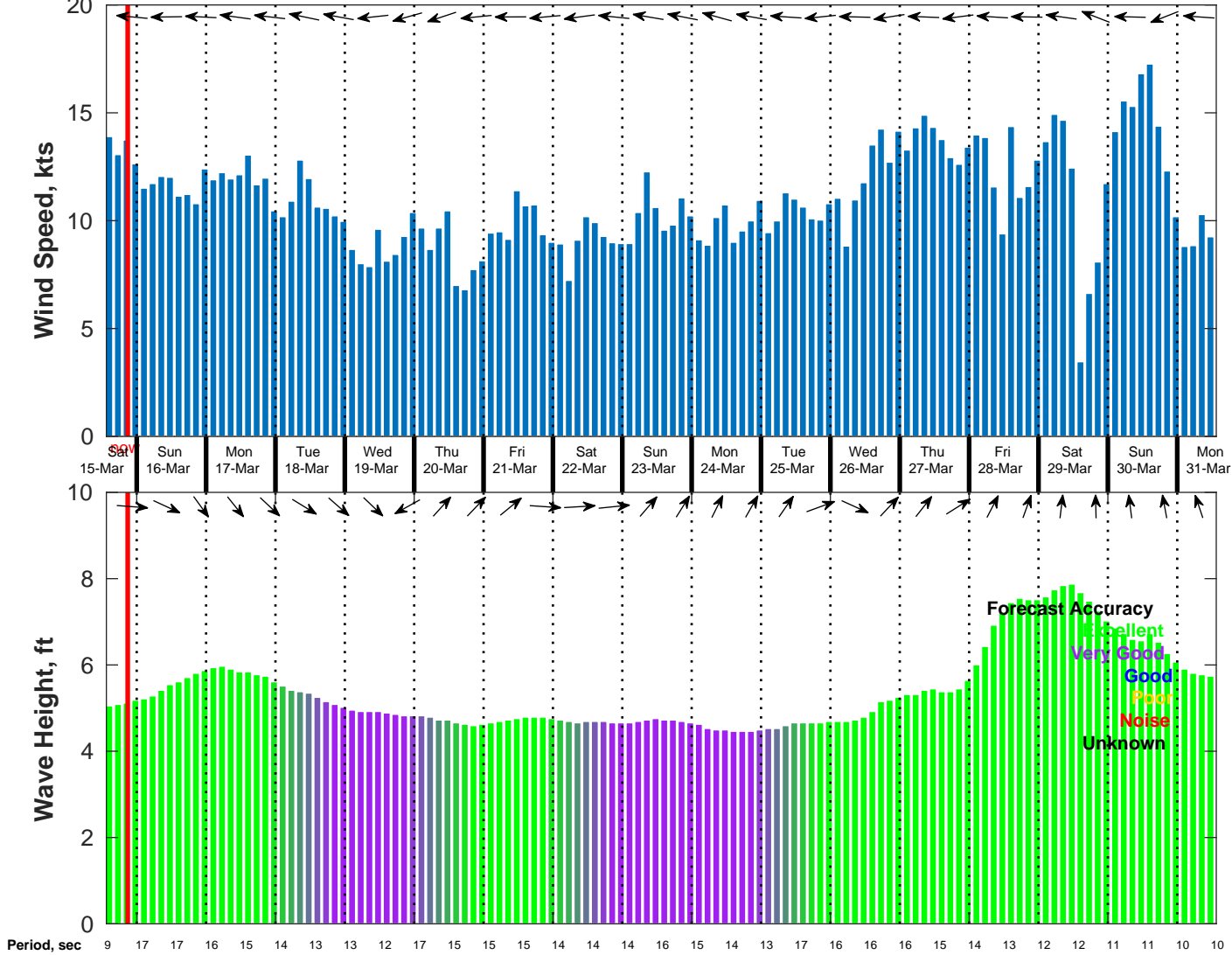
Wind & Wave Forecast for NDBC 51209 from 15-Mar-2025 13:00:00 to 31-Mar-2025 13:00:00
