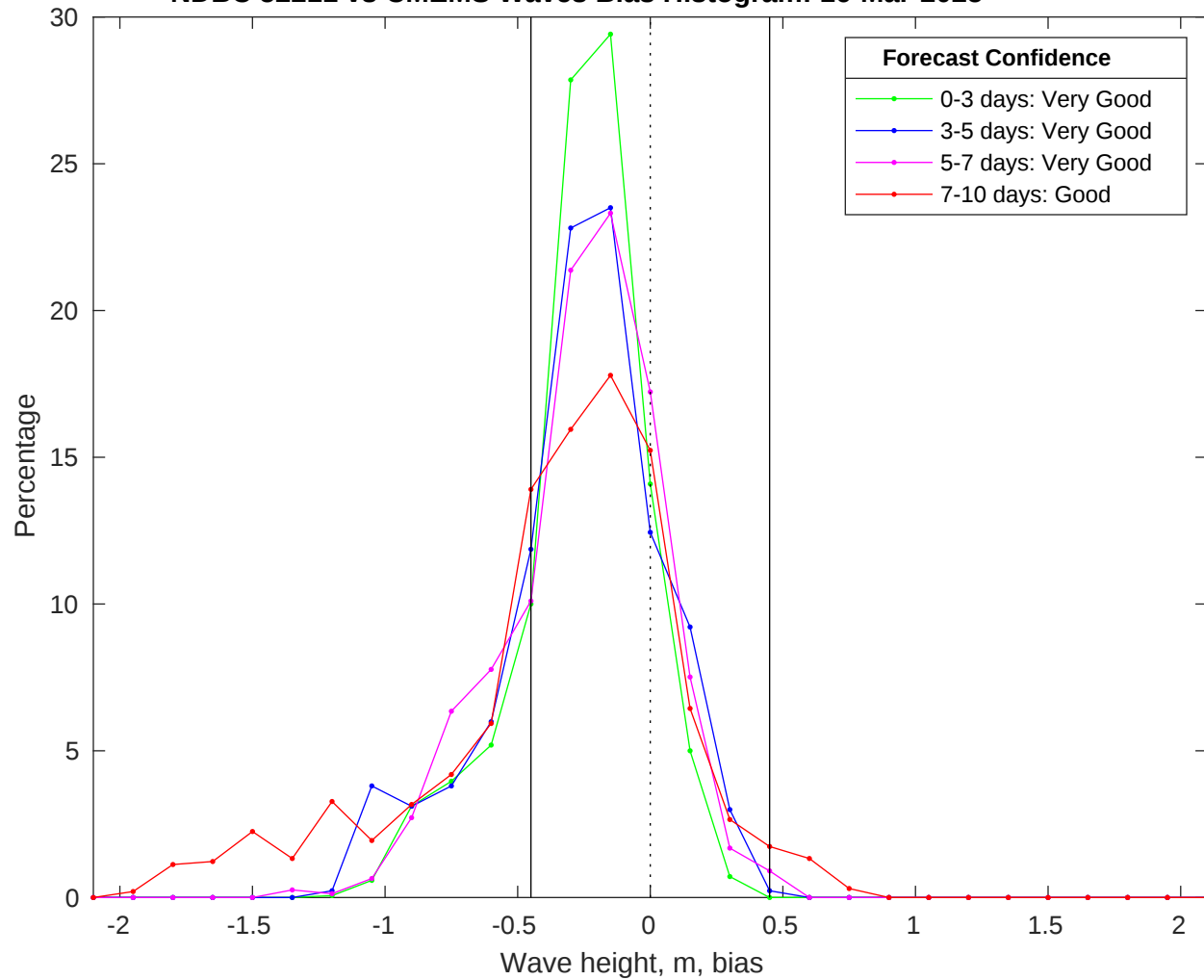
NDBC 52211 vs CMEMS Waves Bias Histogram: 16-Mar-2025
