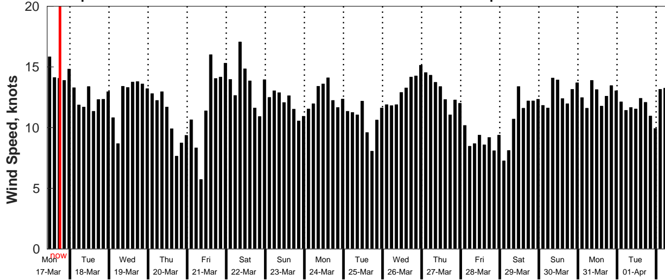
GFS Wind Speed Forecast for NDBC 52211 from 16-Mar-2025 10:00:00 to 01-Apr-2025 10:00:00
