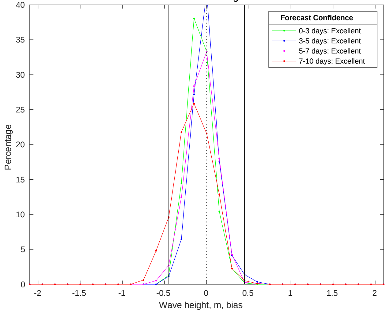
NDBC 52212 vs CMEMS Waves Bias Histogram: 16-Mar-2025
