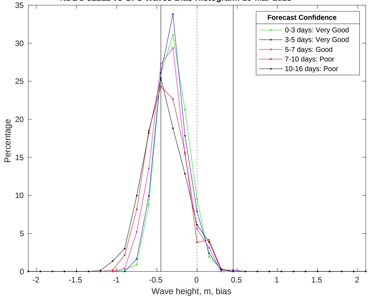
NDBC 52212 vs GFS Waves Bias Histogram: 16-Mar-2025
