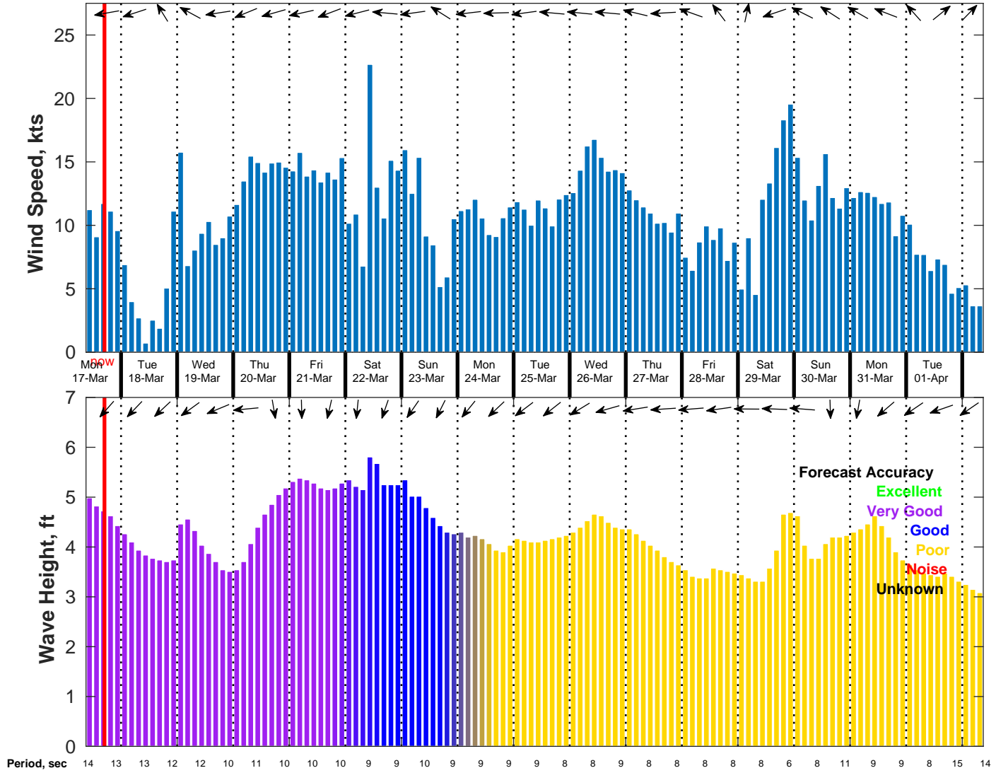
Wind & Wave Forecast for NDBC 52212 from 16-Mar-2025 09:00:00 to 01-Apr-2025 09:00:00
