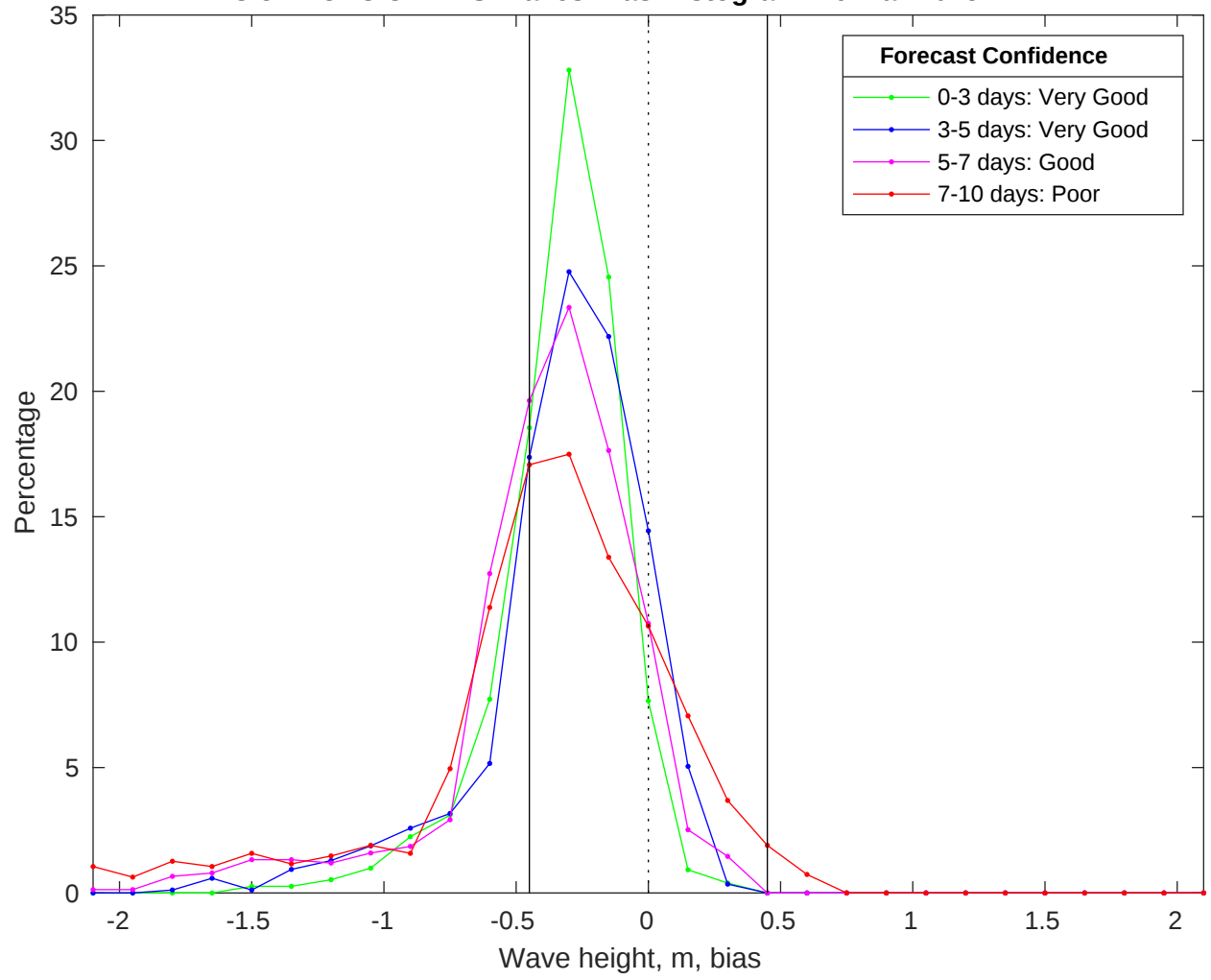
NDBC 52213 vs CMEMS Waves Bias Histogram: 16-Mar-2025
