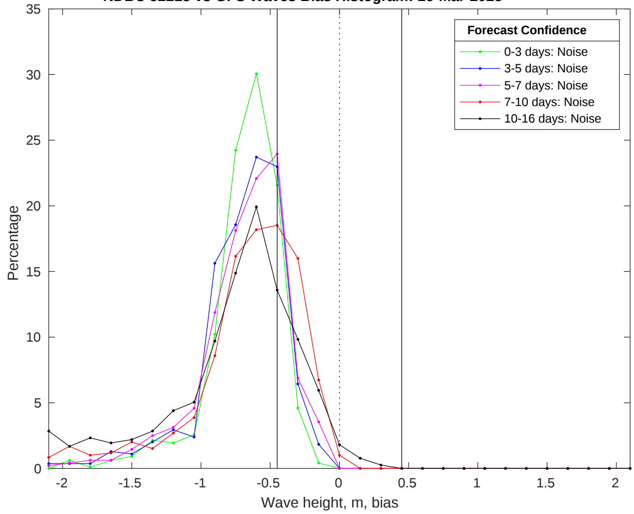
NDBC 52213 vs GFS Waves Bias Histogram: 16-Mar-2025
