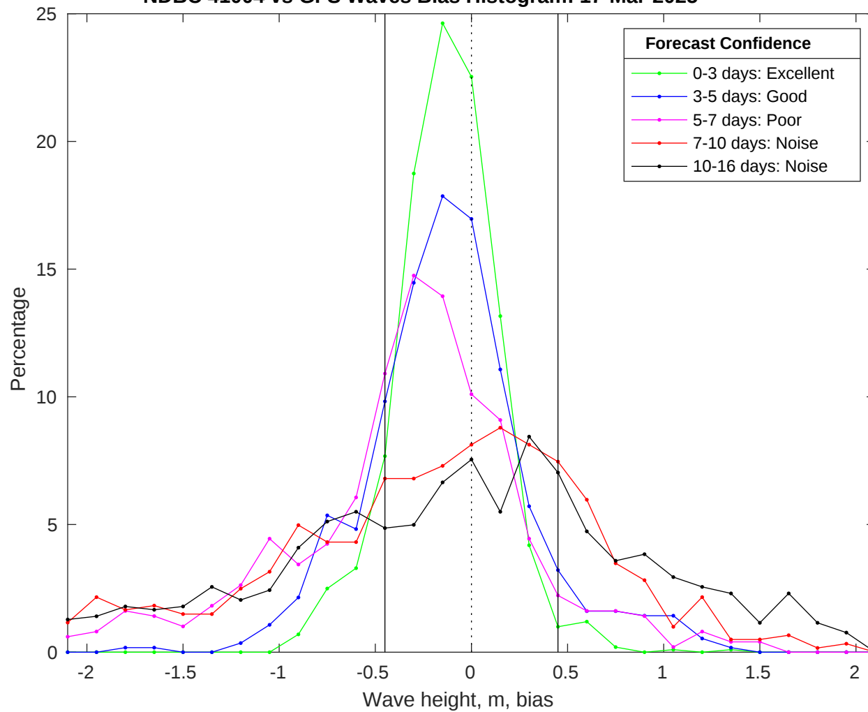
NDBC 41004 vs GFS Waves Bias Histogram: 17-Mar-2025
