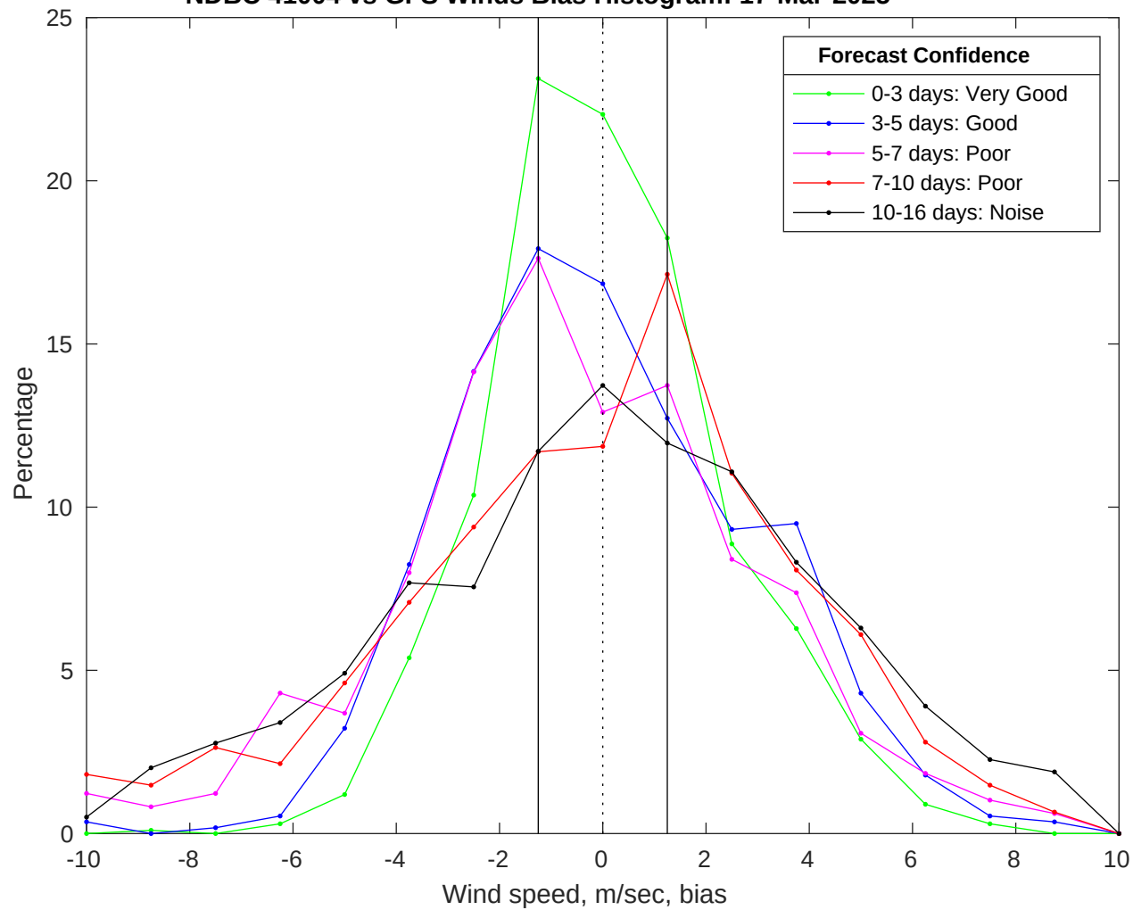
NDBC 41004 vs GFS Winds Bias Histogram: 17-Mar-2025
