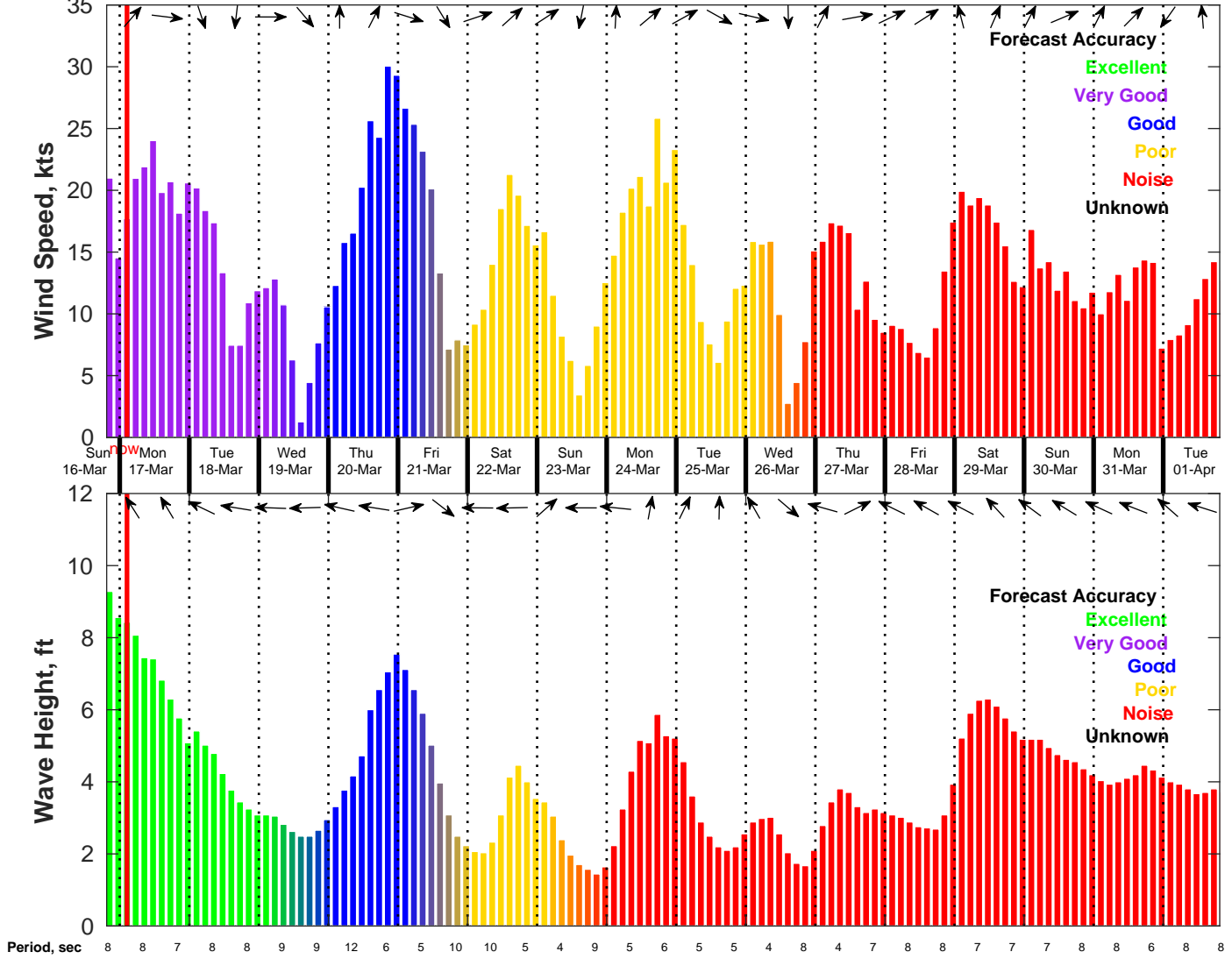
Wind & Wave Forecast for NDBC 41004 from 16-Mar-2025 19:00:00 to 01-Apr-2025 19:00:00
