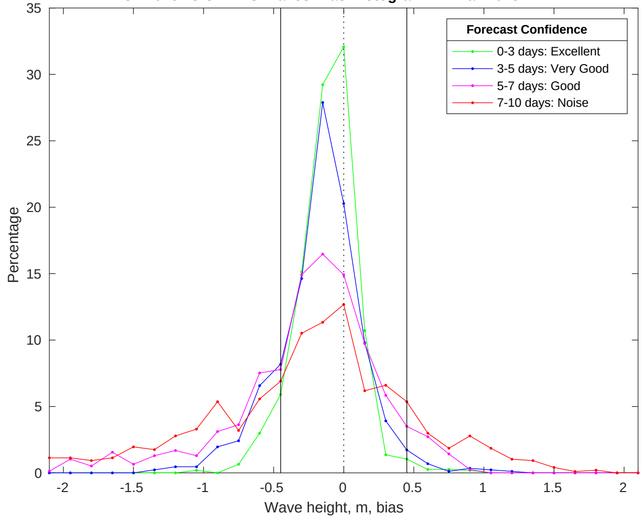
NDBC 41013 vs CMEMS Waves Bias Histogram: 17-Mar-2025
