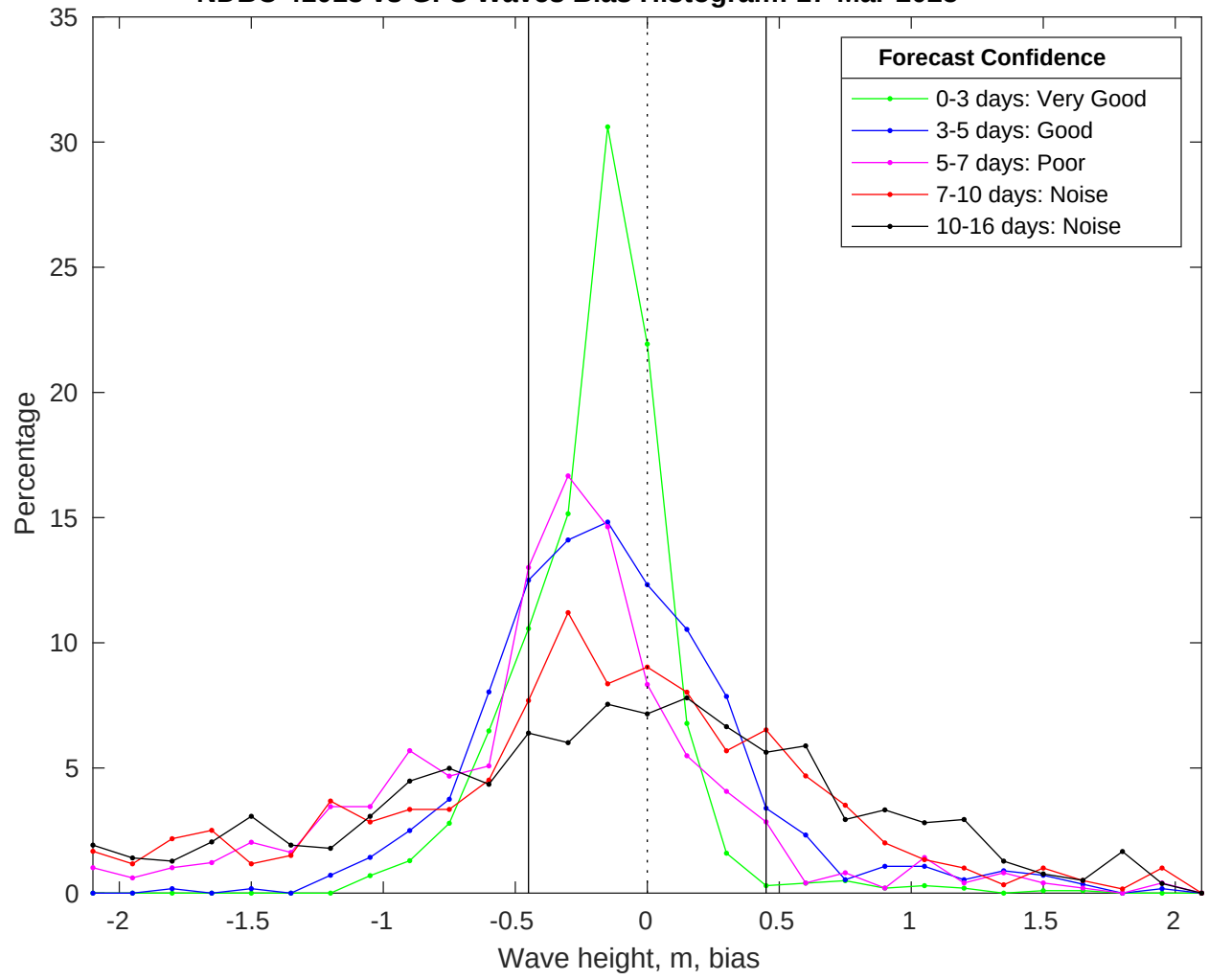
NDBC 41013 vs GFS Waves Bias Histogram: 17-Mar-2025
