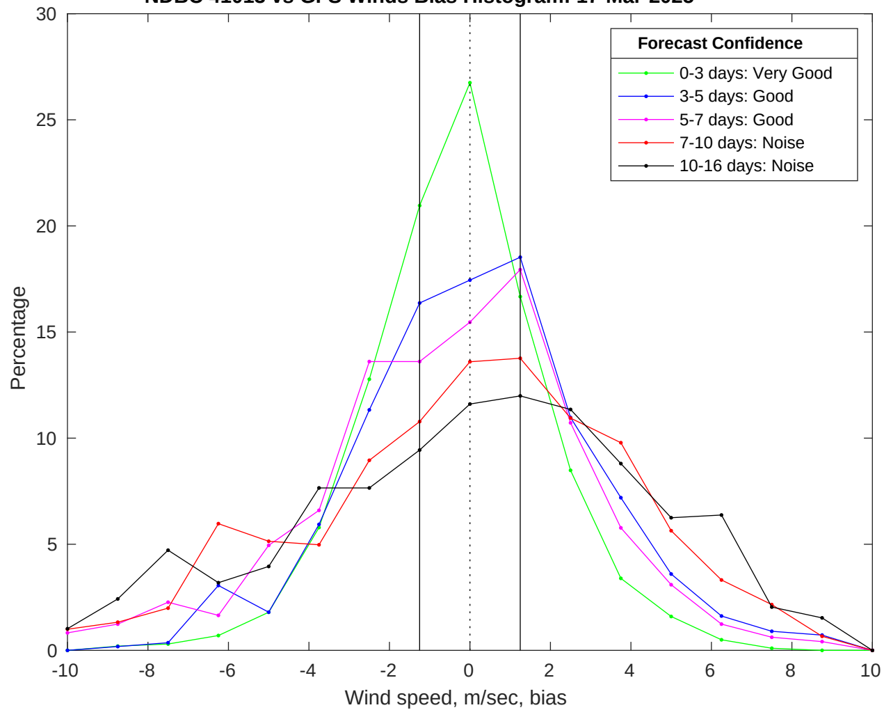
NDBC 41013 vs GFS Winds Bias Histogram: 17-Mar-2025
