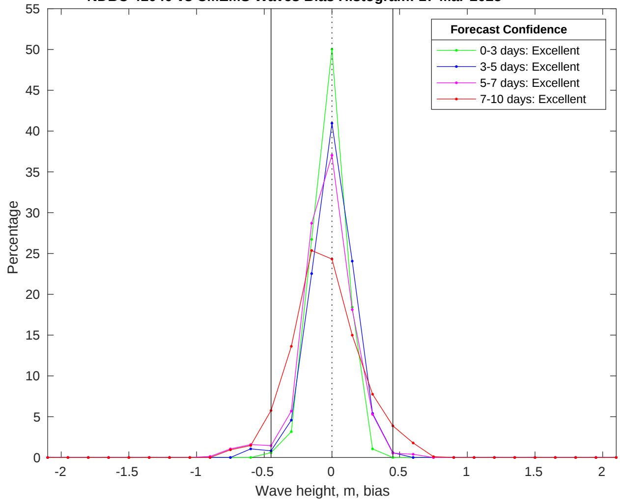
NDBC 41040 vs CMEMS Waves Bias Histogram: 17-Mar-2025
