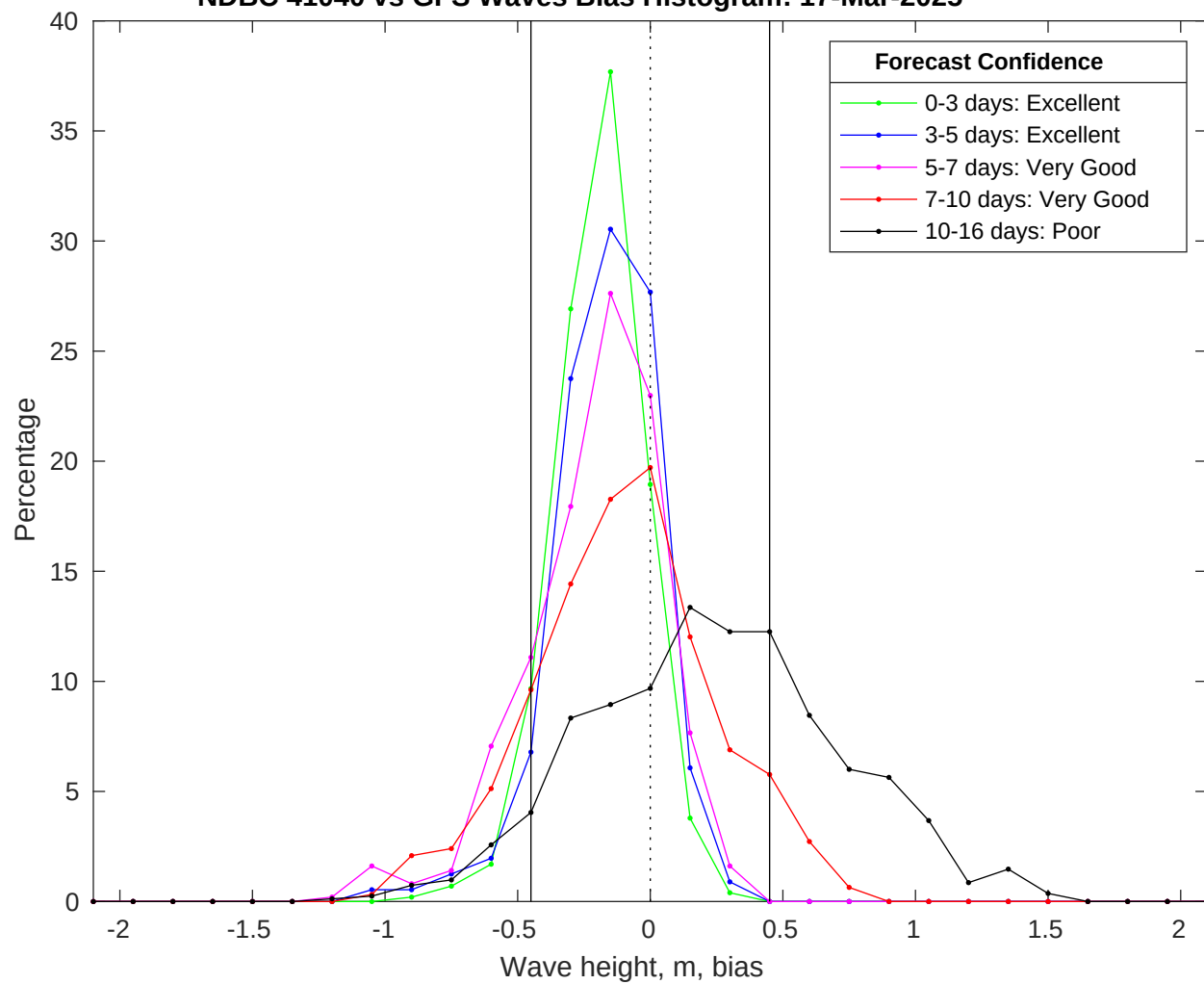
NDBC 41040 vs GFS Waves Bias Histogram: 17-Mar-2025
