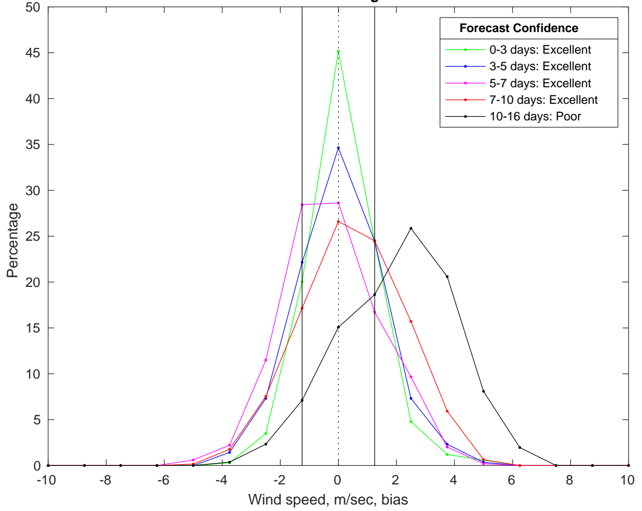
NDBC 41040 vs GFS Winds Bias Histogram: 17-Mar-2025
