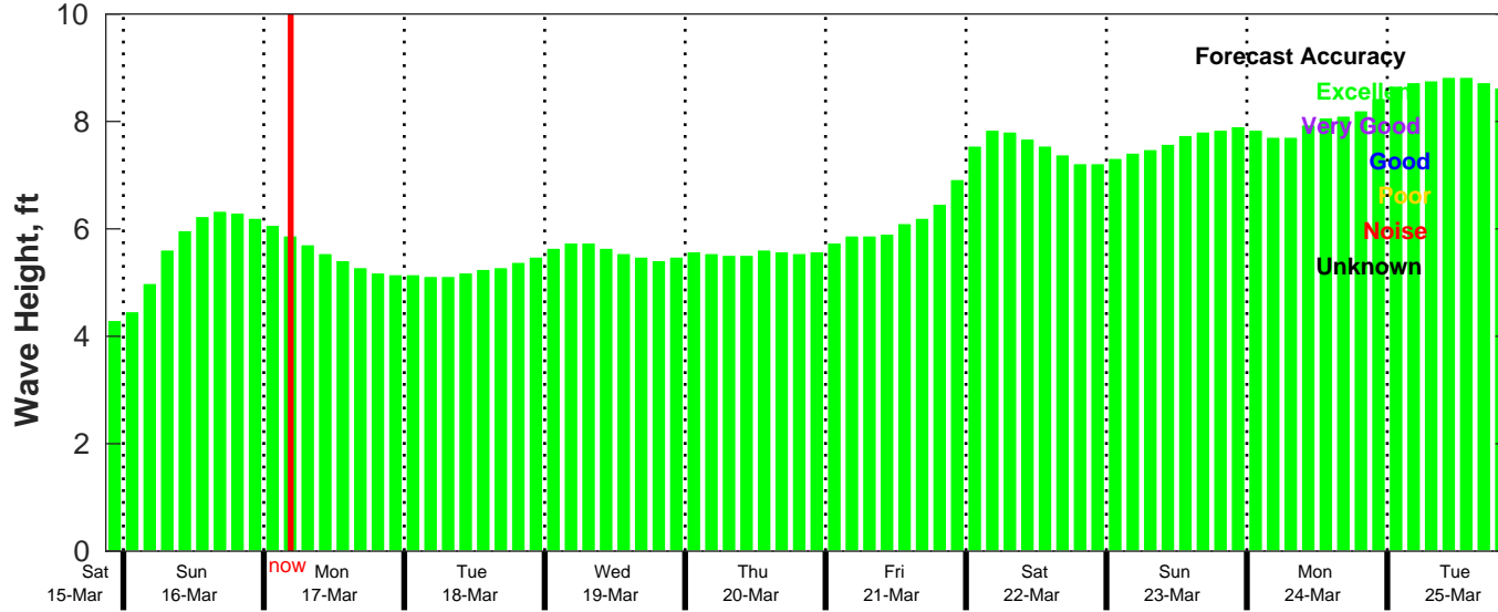
CMEMS Wave Forecast for NDBC 41040 from 15-Mar-2025 21:00:00 to 25-Mar-2025 21:00:00
