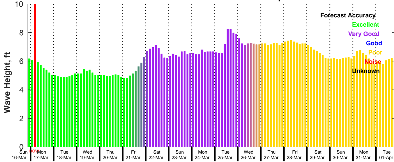
GFS Wave Forecast for NDBC 41040 from 16-Mar-2025 21:00:00 to 01-Apr-2025 21:00:00
