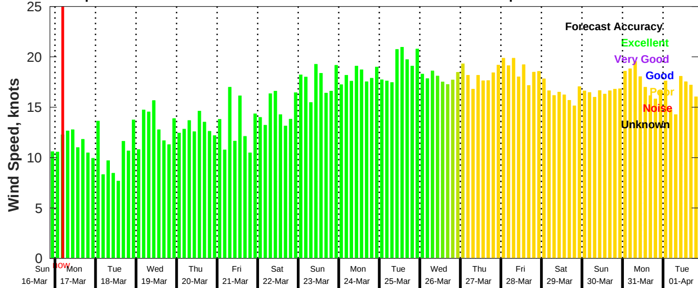
GFS Wind Speed Forecast for NDBC 41040 from 16-Mar-2025 21:00:00 to 01-Apr-2025 21:00:00
