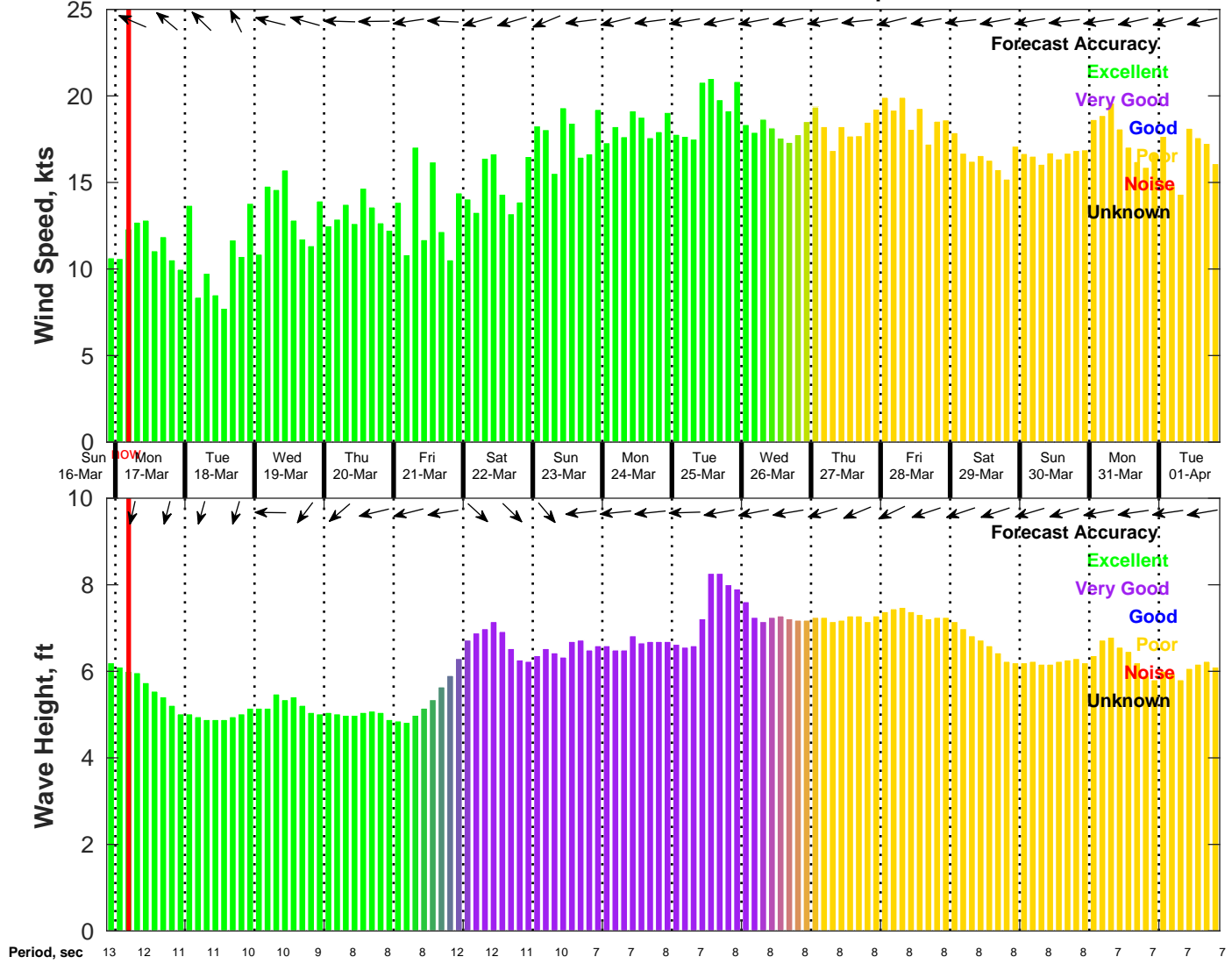
Wind & Wave Forecast for NDBC 41040 from 16-Mar-2025 21:00:00 to 01-Apr-2025 21:00:00
