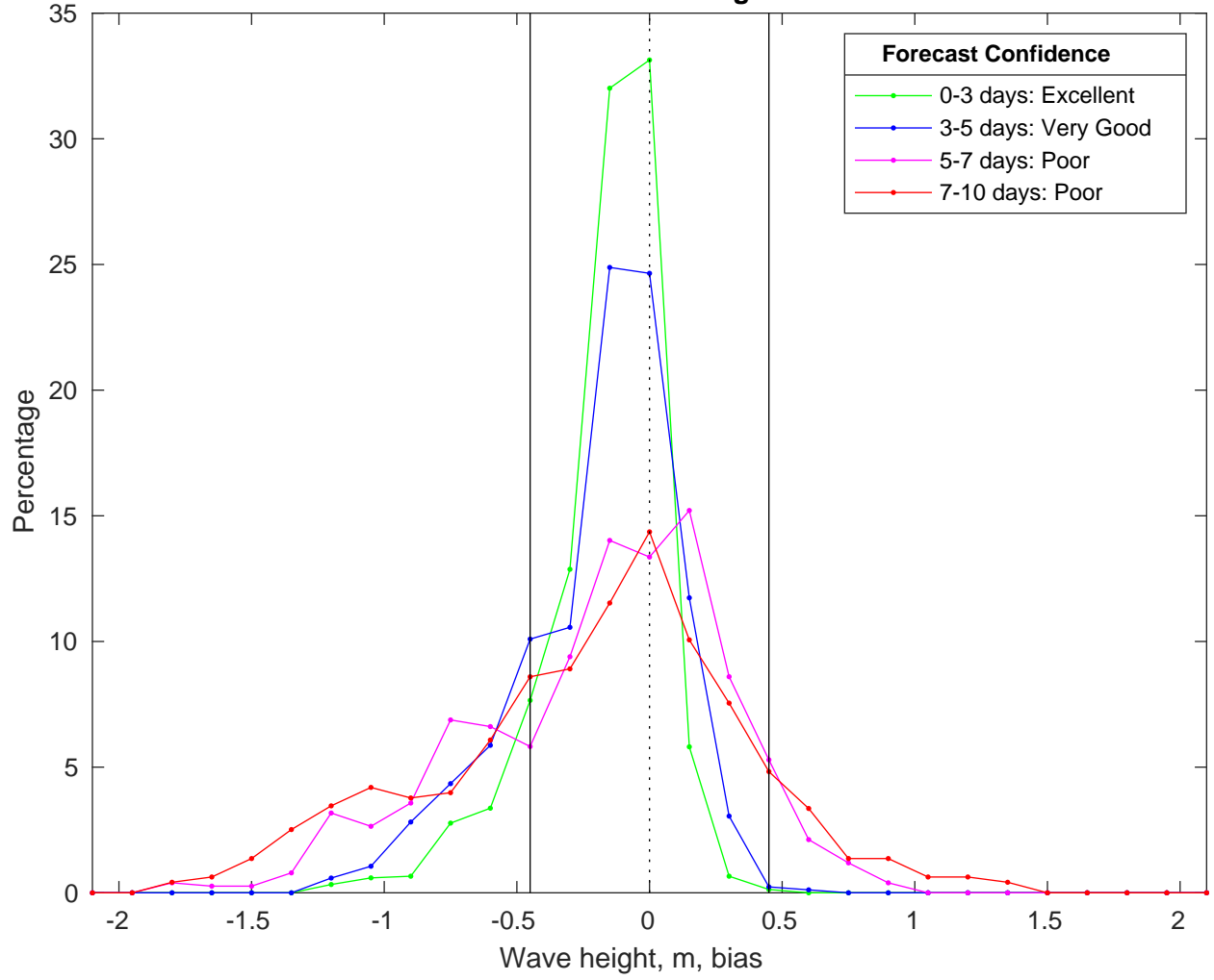
NDBC 42019 vs CMEMS Waves Bias Histogram: 17-Mar-2025
